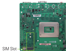
M.2 Key B ▲ Rear view (2242/3042/3052)
